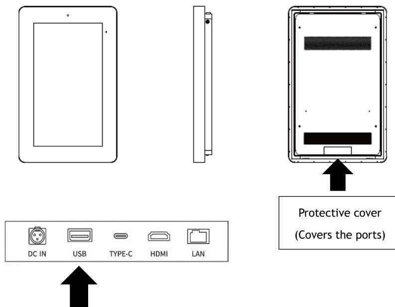
Figure 1 Position of USB ports
